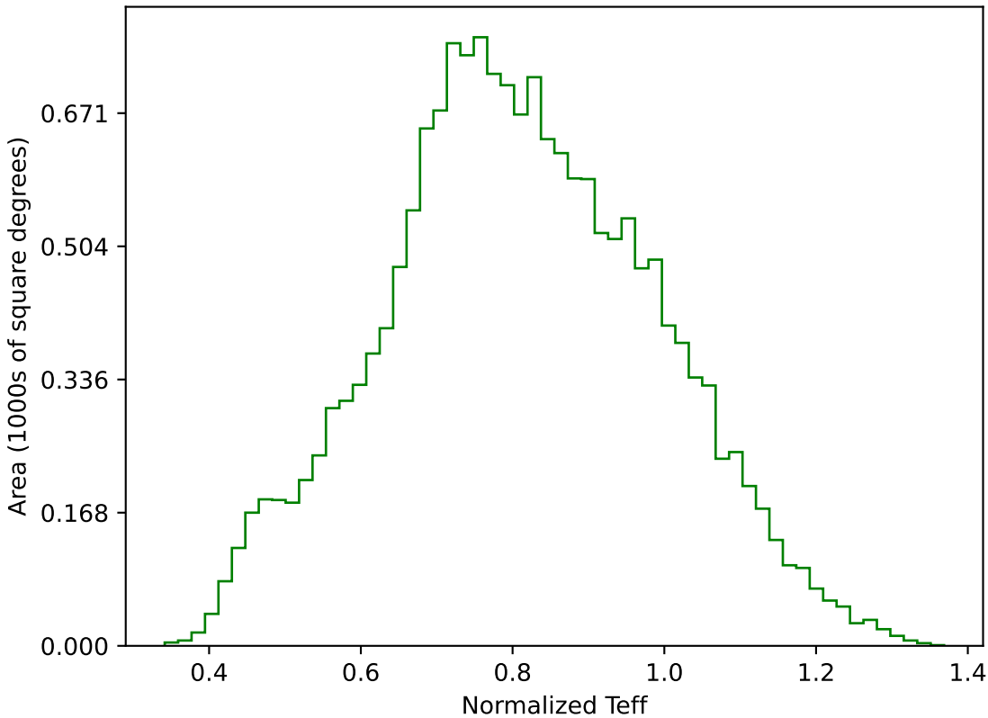
ddf_half_v3.4_10yrs WFD g band: Normalized Teff
