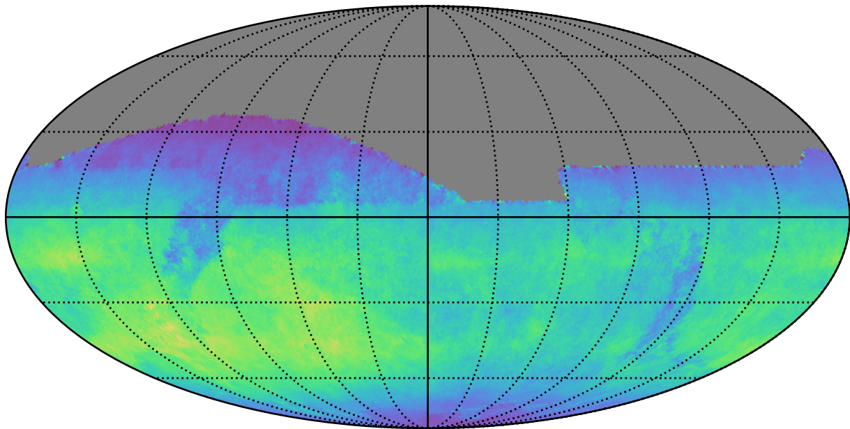
ddf_half_v3.4_10yrs All sky z band: Normalized Teff
