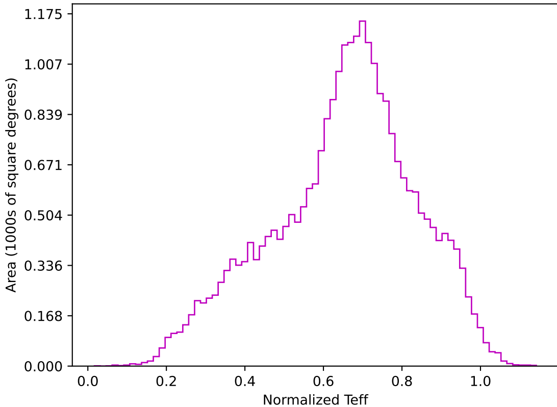
ddf_half_v3.4_10yrs All sky z band: Normalized Teff
