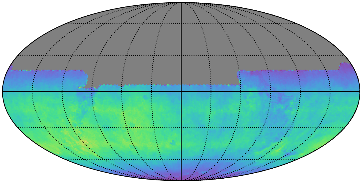
ddf_half_v3.4_10yrs All sky y band: Normalized Teff
