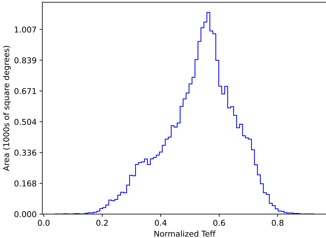
ddf_half_v3.4_10yrs All sky y band: Normalized Teff
