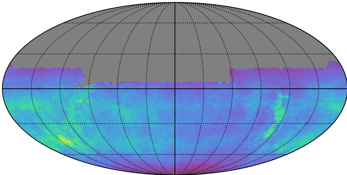
ddf_half_v3.4_10yrs All sky u band: Normalized Teff
