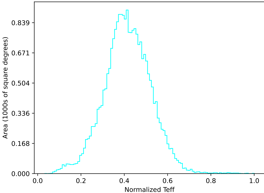
ddf_half_v3.4_10yrs All sky u band: Normalized Teff
