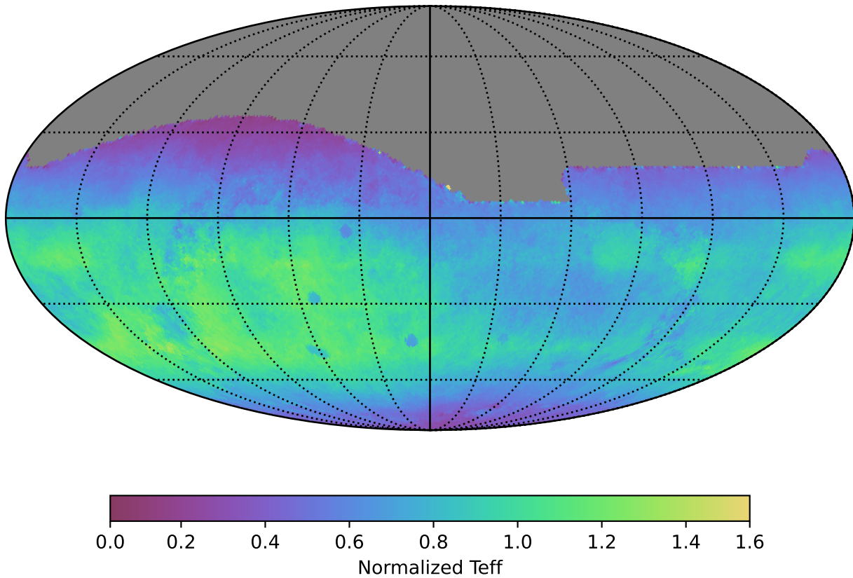
ddf_half_v3.4_10yrs All sky r band: Normalized Teff
