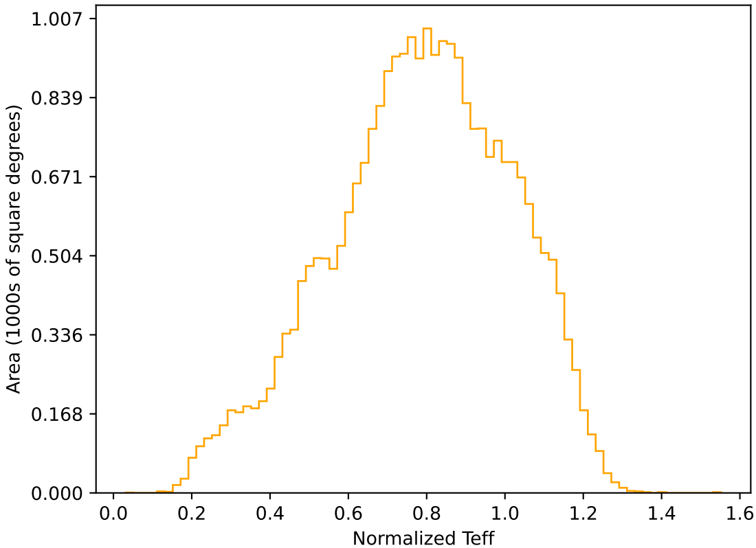
ddf_half_v3.4_10yrs All sky r band: Normalized Teff
