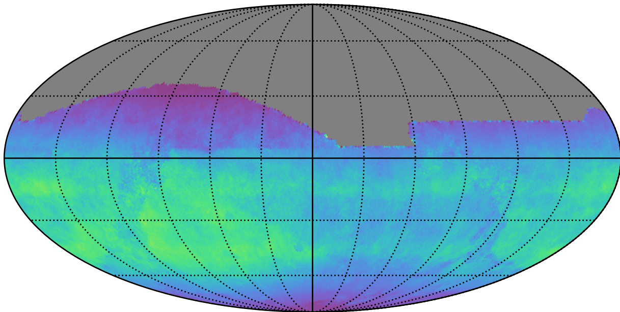
ddf_half_v3.4_10yrs All sky i band: Normalized Teff
