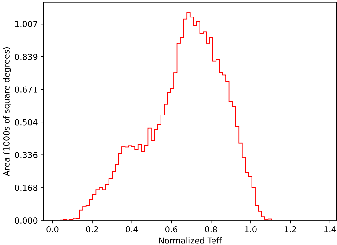
ddf_half_v3.4_10yrs All sky i band: Normalized Teff
