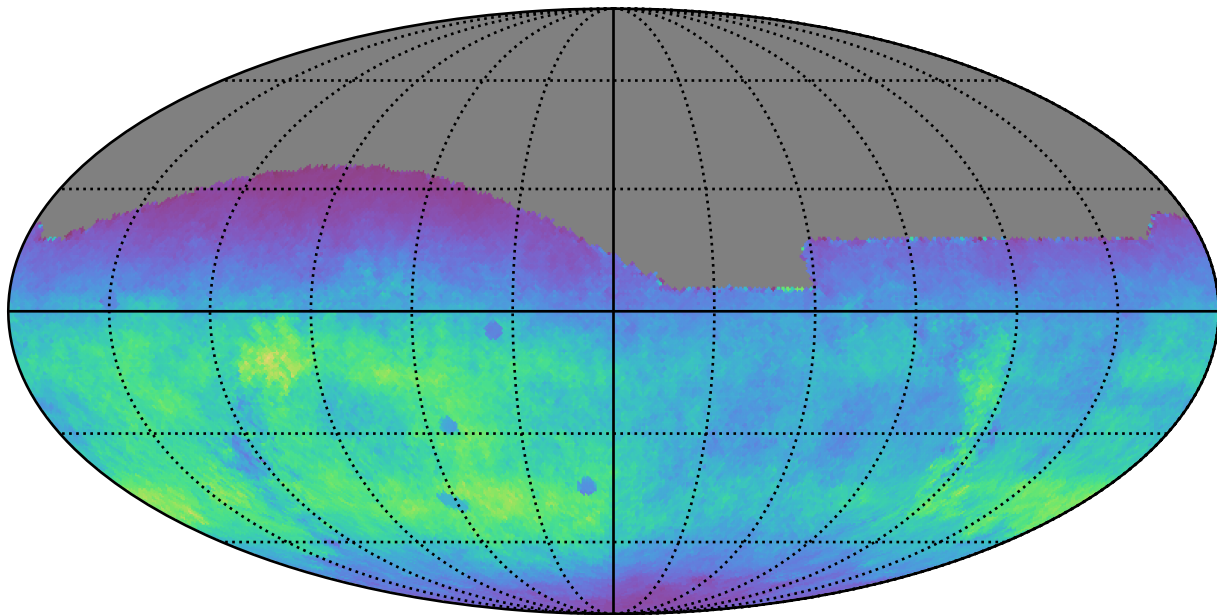
ddf_half_v3.4_10yrs All sky g band: Normalized Teff
