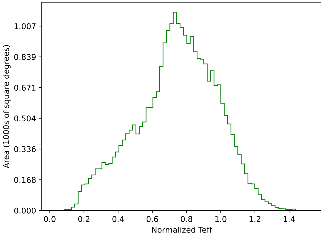
ddf_half_v3.4_10yrs All sky g band: Normalized Teff
