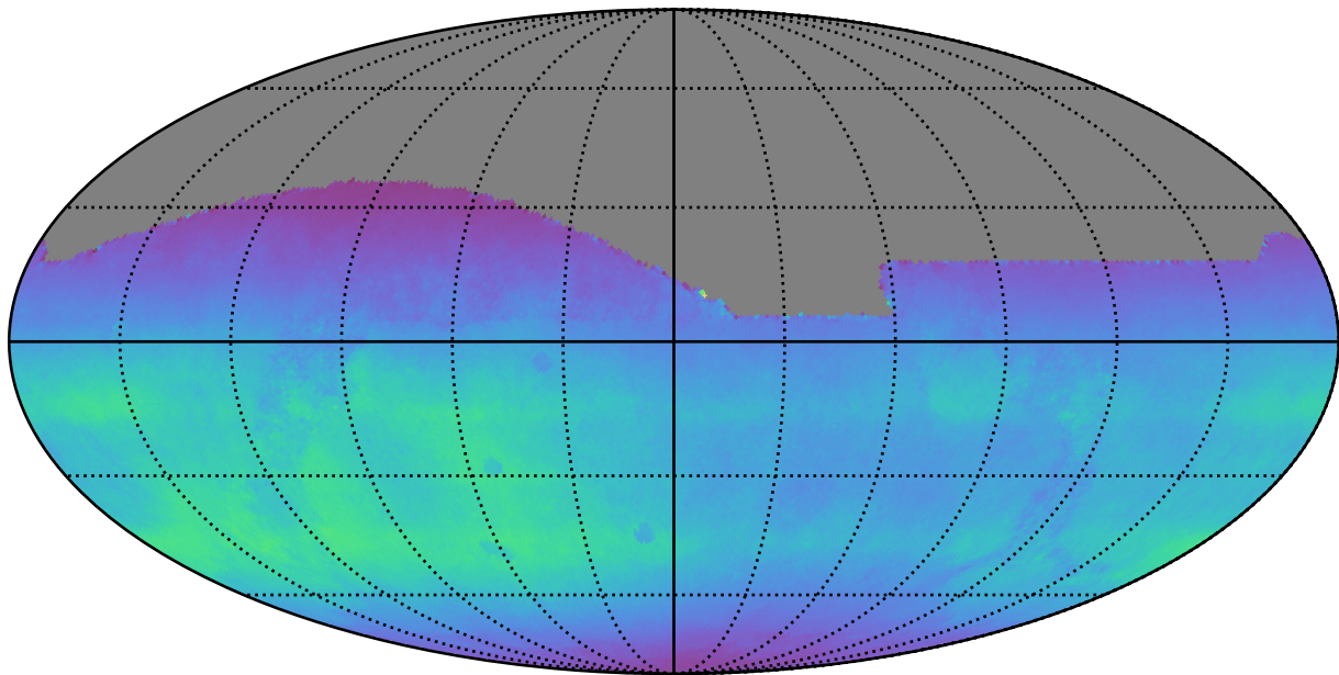
ddf_half_v3.4_10yrs All sky all bands: Normalized Teff
