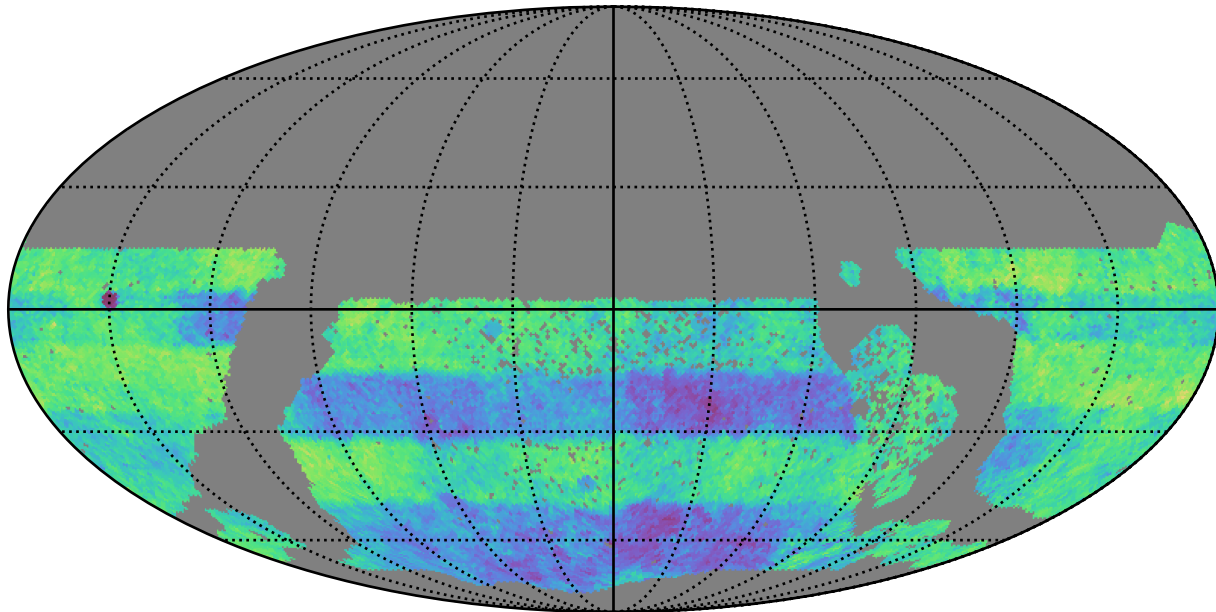
ddf_half_v3.4_10yrs WFD: Normalized Proper Motion Uncert @ 24.0
