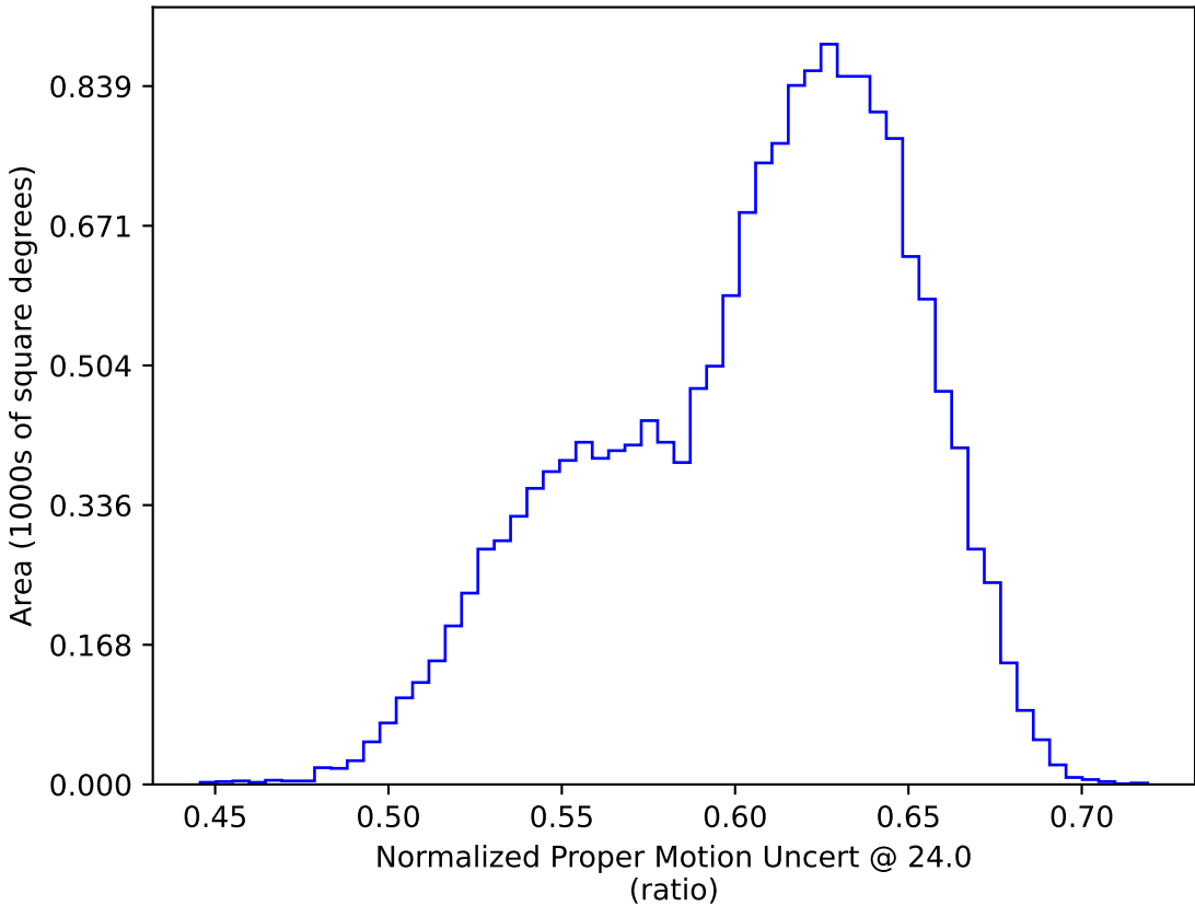
ddf_half_v3.4_10yrs WFD: Normalized Proper Motion Uncert @ 24.0
