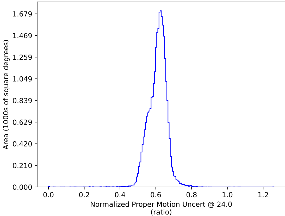
ddf_half_v3.4_10yrs All sky: Normalized Proper Motion Uncert @ 24.0
