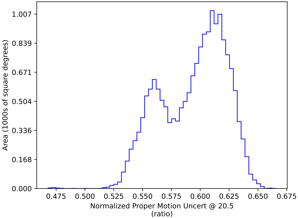
ddf_half_v3.4_10yrs WFD: Normalized Proper Motion Uncert @ 20.5
