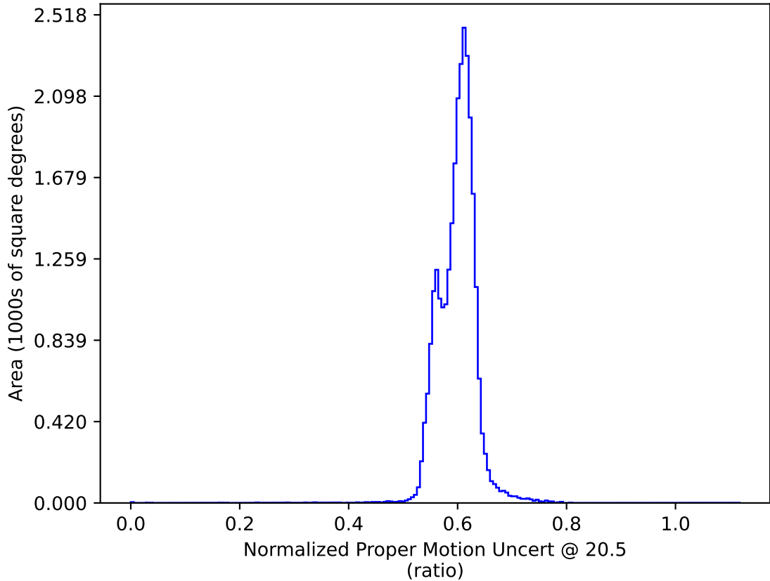
ddf_half_v3.4_10yrs All sky: Normalized Proper Motion Uncert @ 20.5
