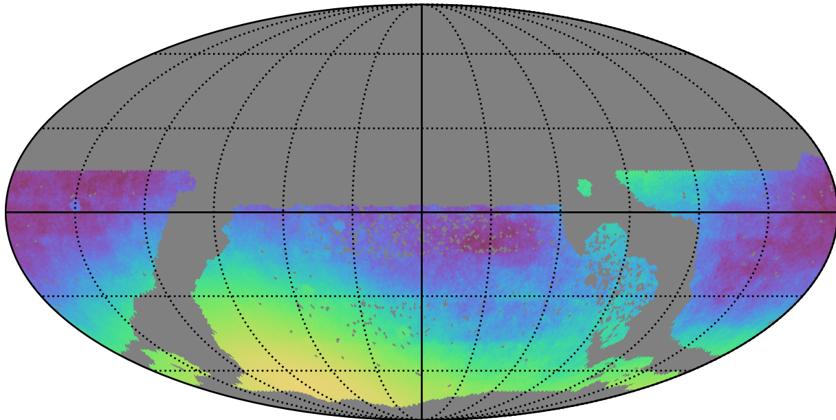
ddf_half_v3.4_10yrs WFD: Normalized Parallax Uncert @ 24.0
