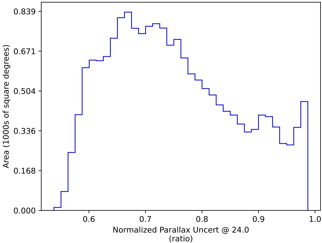
ddf_half_v3.4_10yrs WFD: Normalized Parallax Uncert @ 24.0
