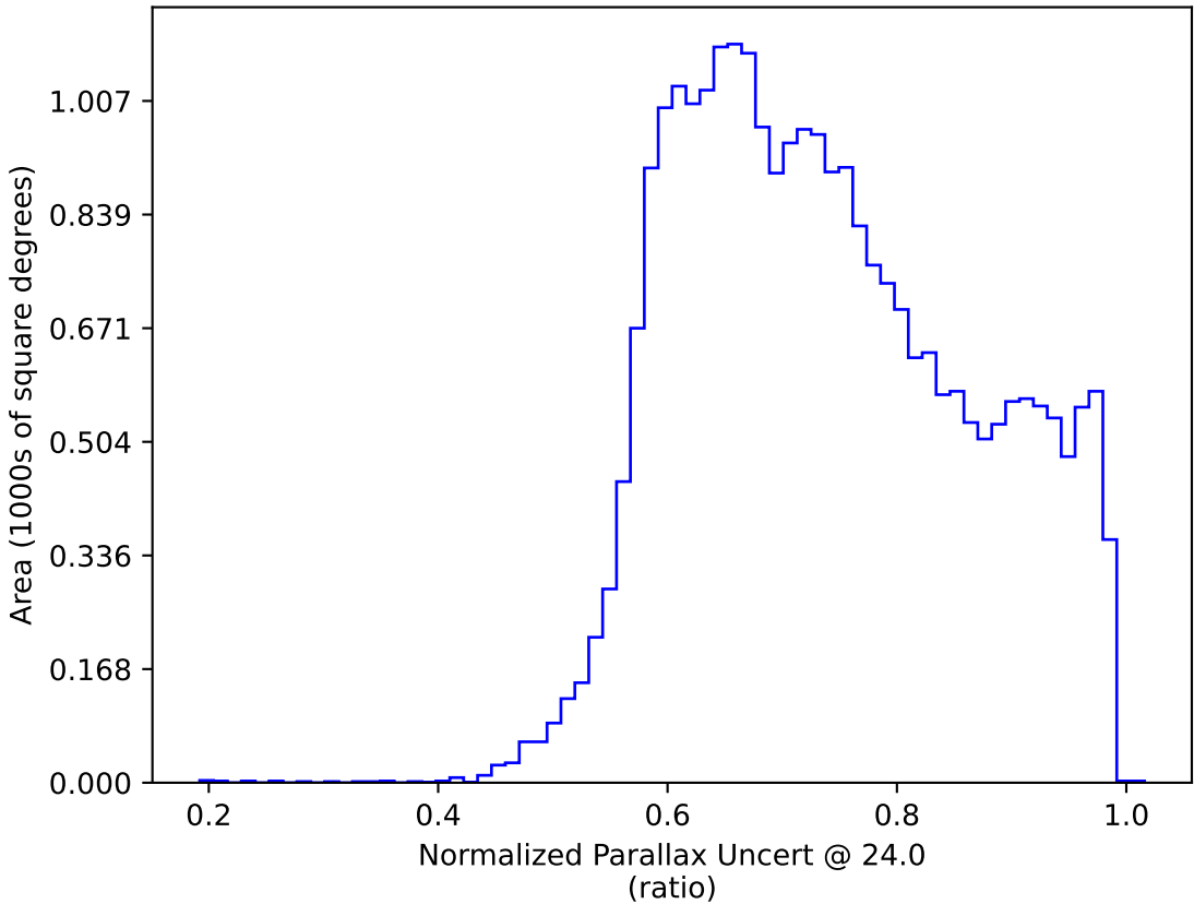
ddf_half_v3.4_10yrs All sky: Normalized Parallax Uncert @ 24.0
