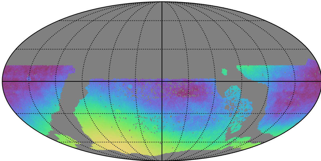
ddf_half_v3.4_10yrs WFD: Normalized Parallax Uncert @ 22.4
