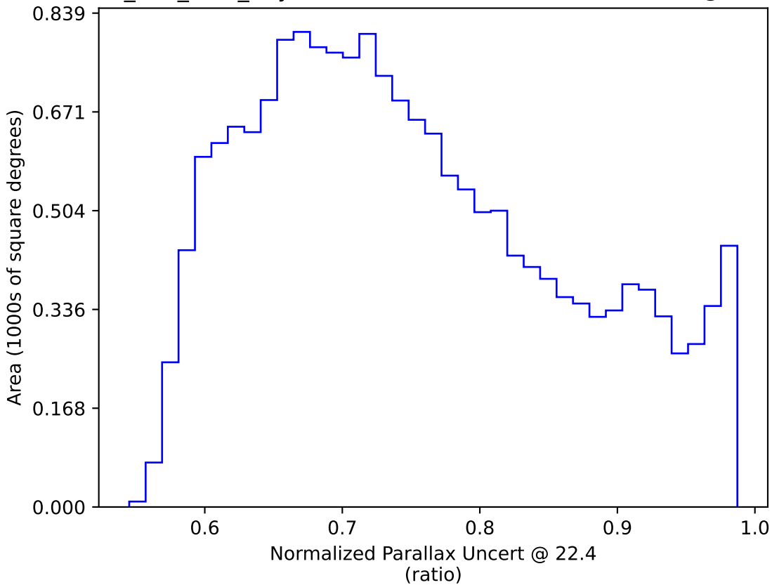
ddf_half_v3.4_10yrs WFD: Normalized Parallax Uncert @ 22.4
