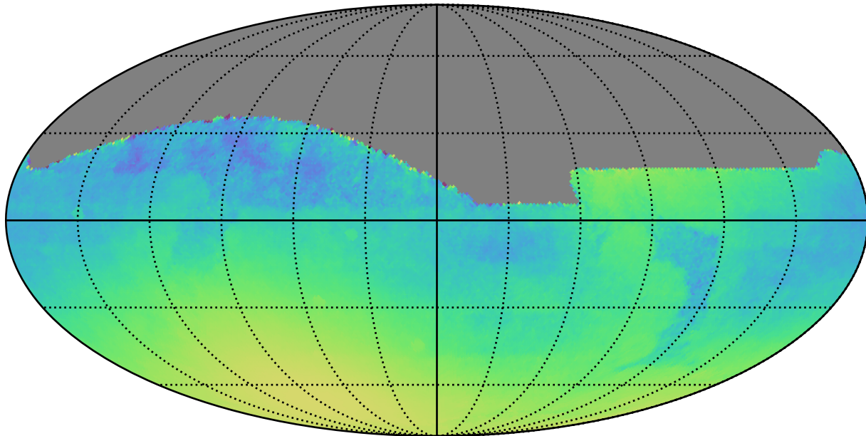
ddf_half_v3.4_10yrs All sky: Normalized Parallax Uncert @ 22.4
