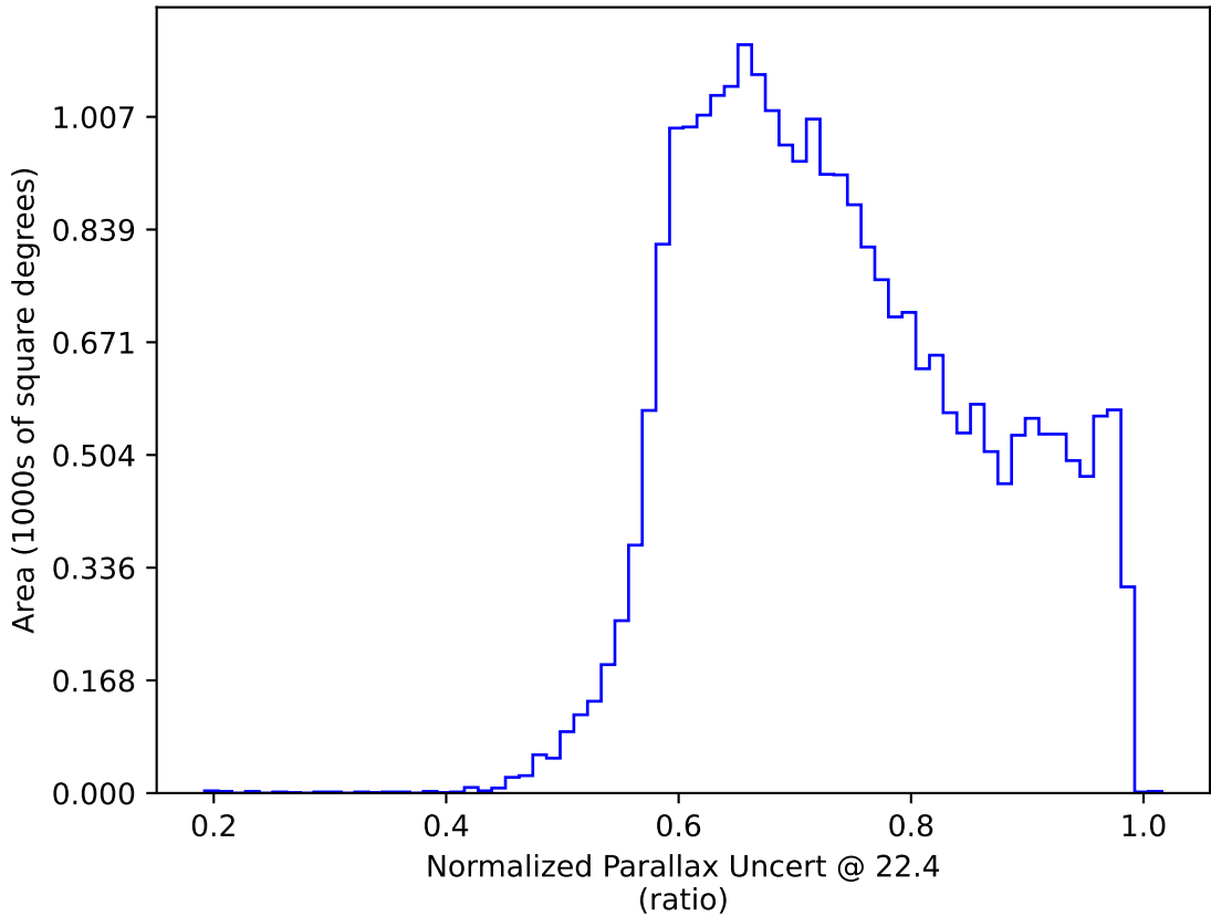
ddf_half_v3.4_10yrs All sky: Normalized Parallax Uncert @ 22.4
