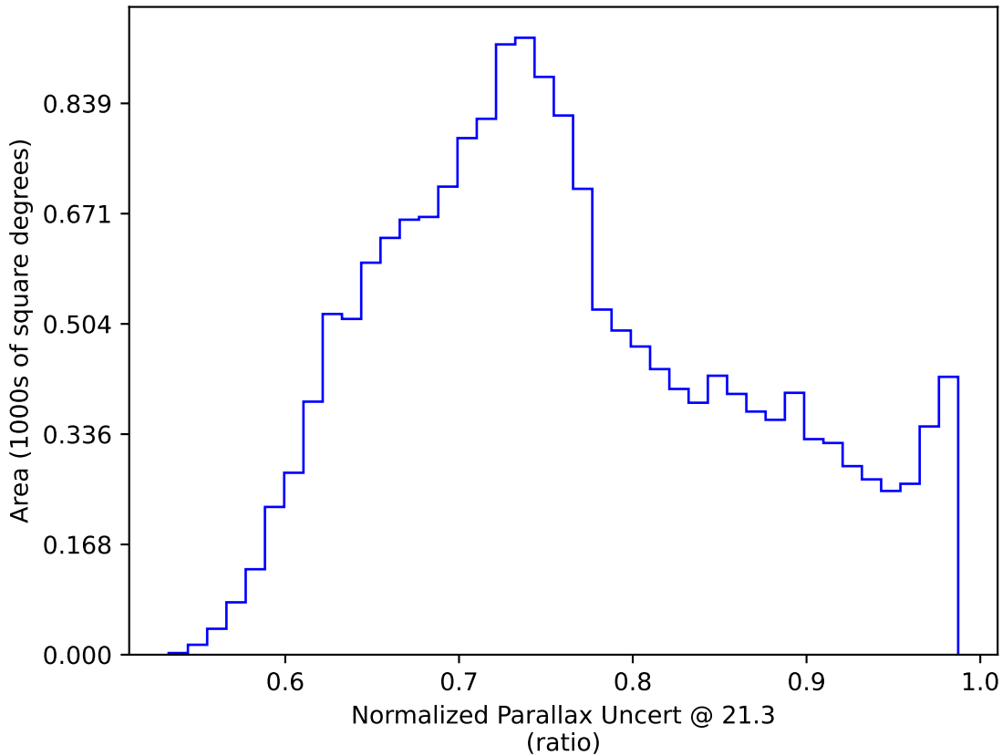
ddf_half_v3.4_10yrs WFD y band only: Normalized Parallax Uncert @ 21.3
