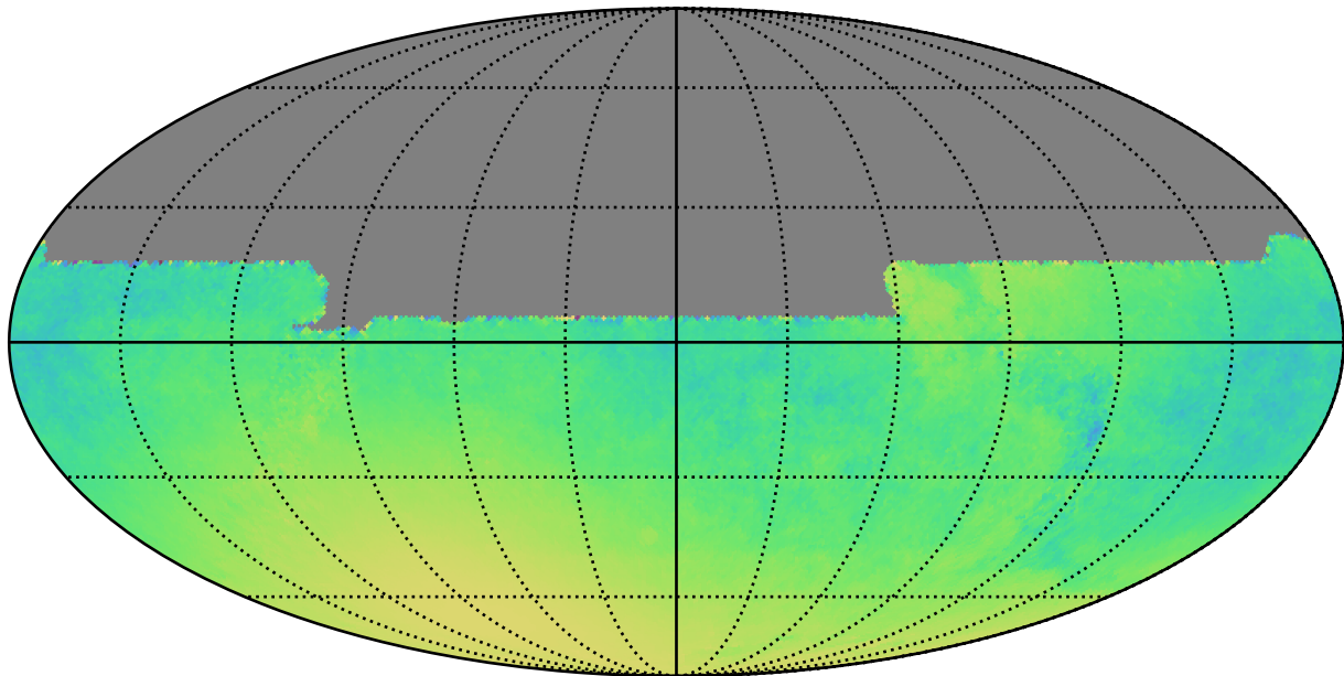
ddf_half_v3.4_10yrs All sky y band only: Normalized Parallax Uncert @ 21.3
