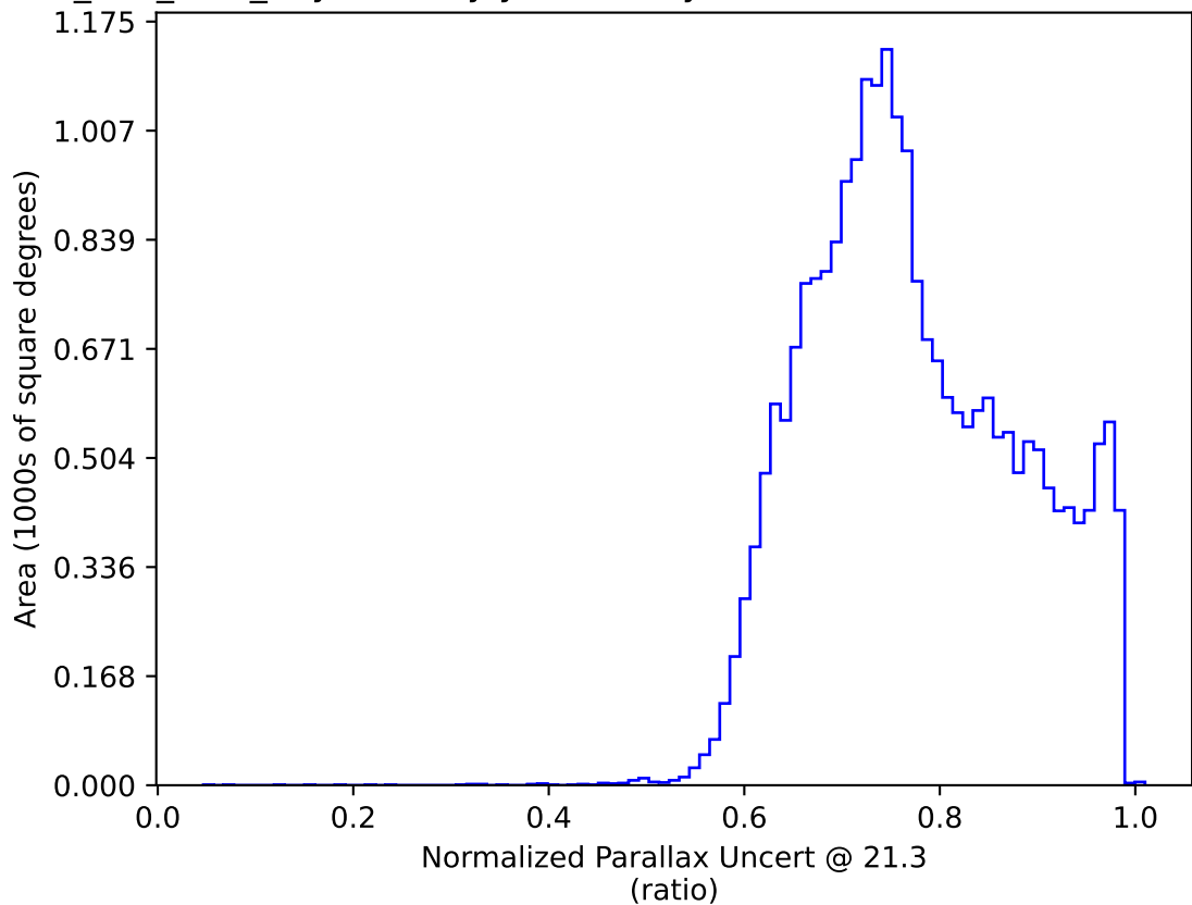
ddf_half_v3.4_10yrs All sky y band only: Normalized Parallax Uncert @ 21.3
