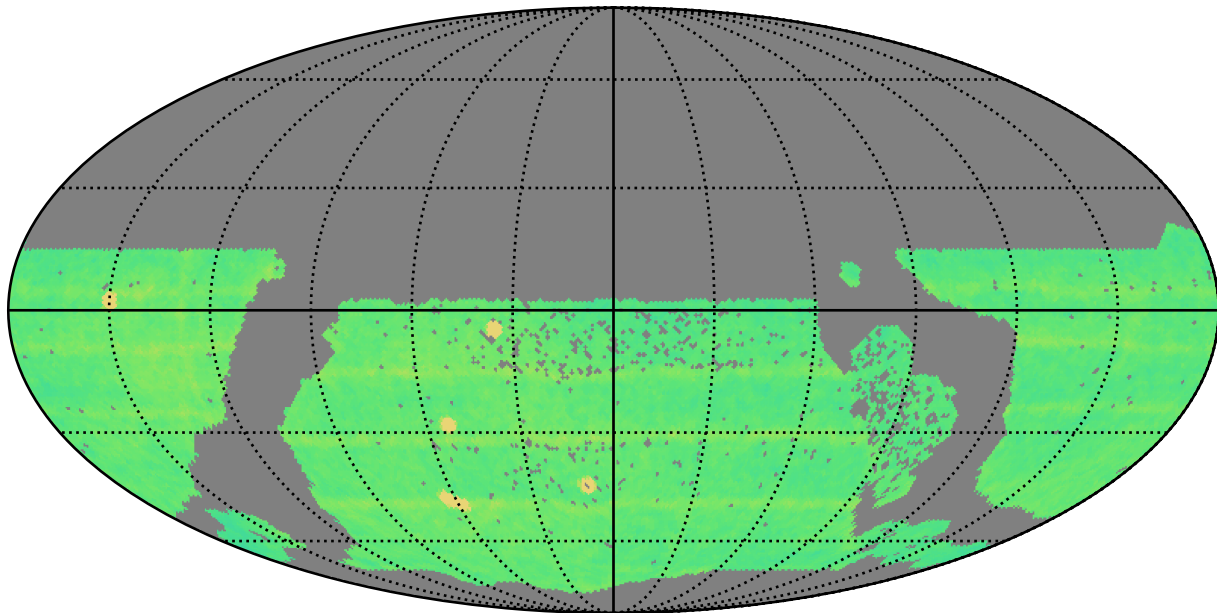
ddf_half_v3.4_10yrs WFD all bands: N Unique Nights
