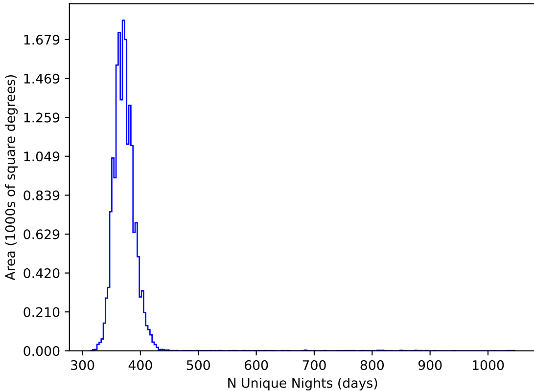
ddf_half_v3.4_10yrs WFD all bands: N Unique Nights
