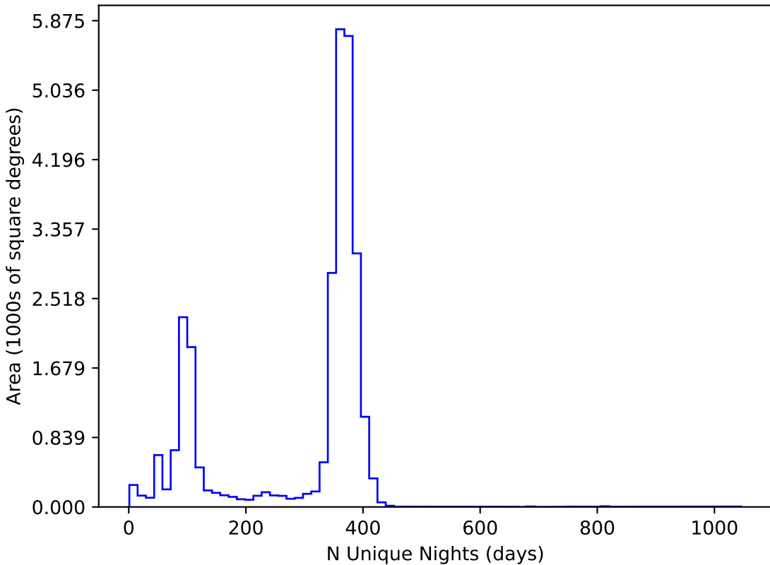
ddf_half_v3.4_10yrs All sky all bands: N Unique Nights
