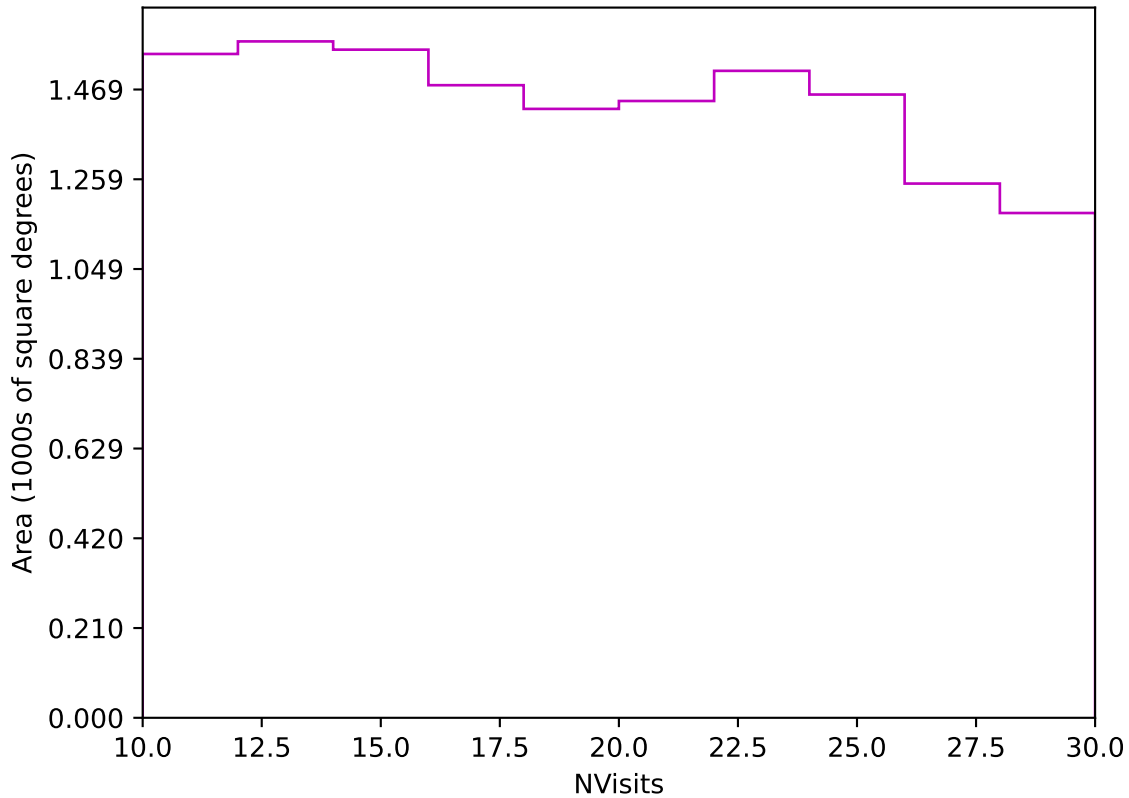
ddf_half_v3.4_10yrs Yr 3-4 z band: NVisits
