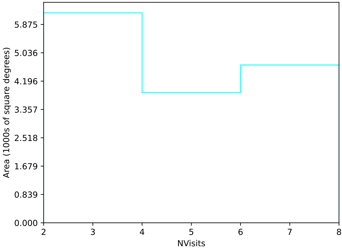
ddf_half_v3.4_10yrs Yr 3-4 u band: NVisits
