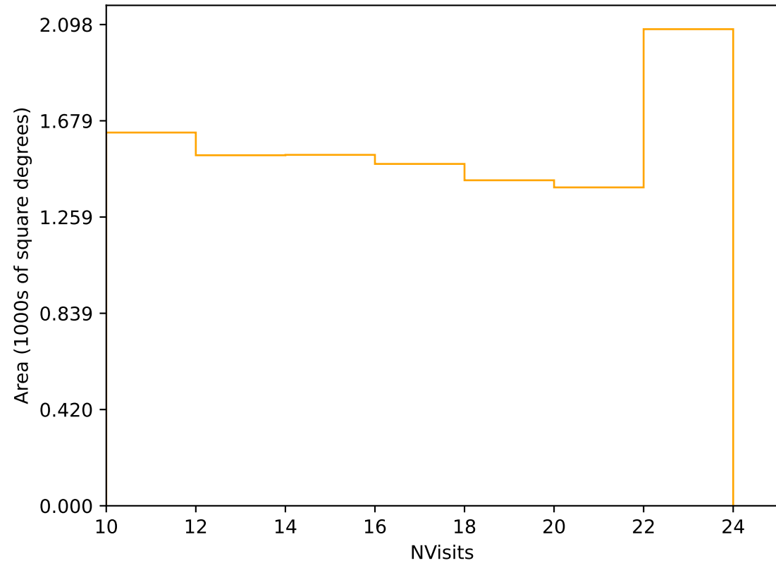
ddf_half_v3.4_10yrs Yr 3-4 r band: NVisits
