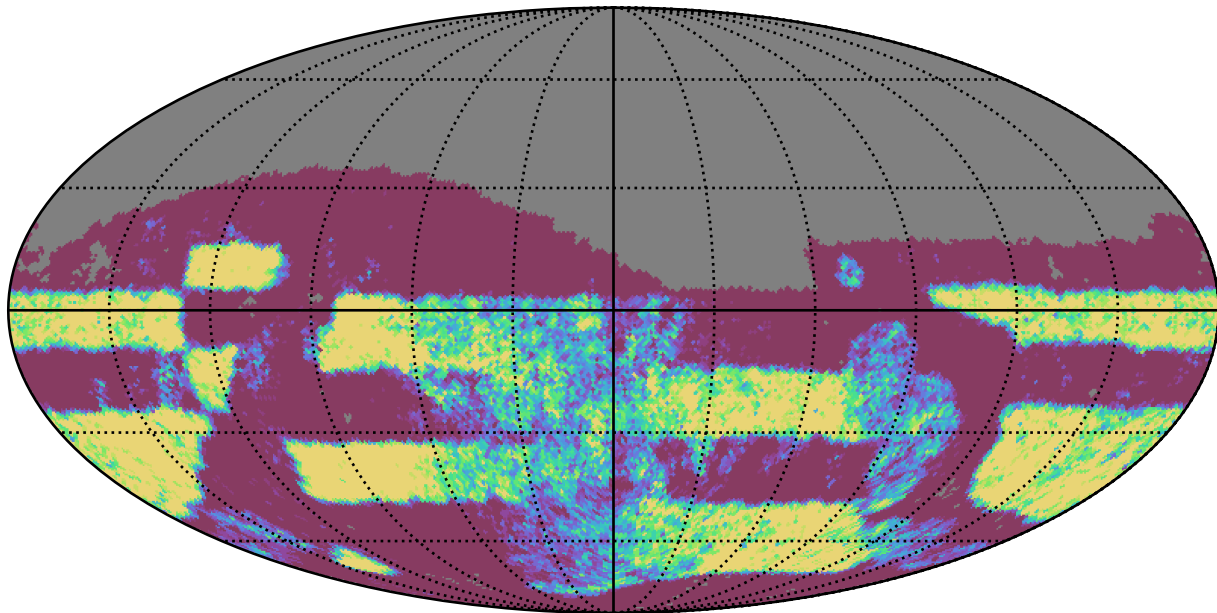
ddf_half_v3.4_10yrs Yr 3-4 i band: NVisits
