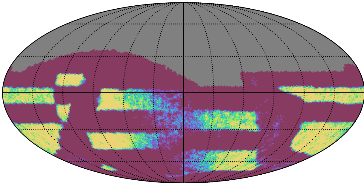
ddf_half_v3.4_10yrs Yr 3-4 all bands: NVisits
