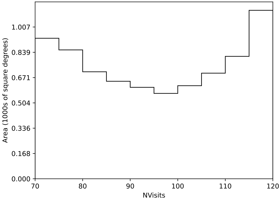
ddf_half_v3.4_10yrs Yr 3-4 all bands: NVisits
