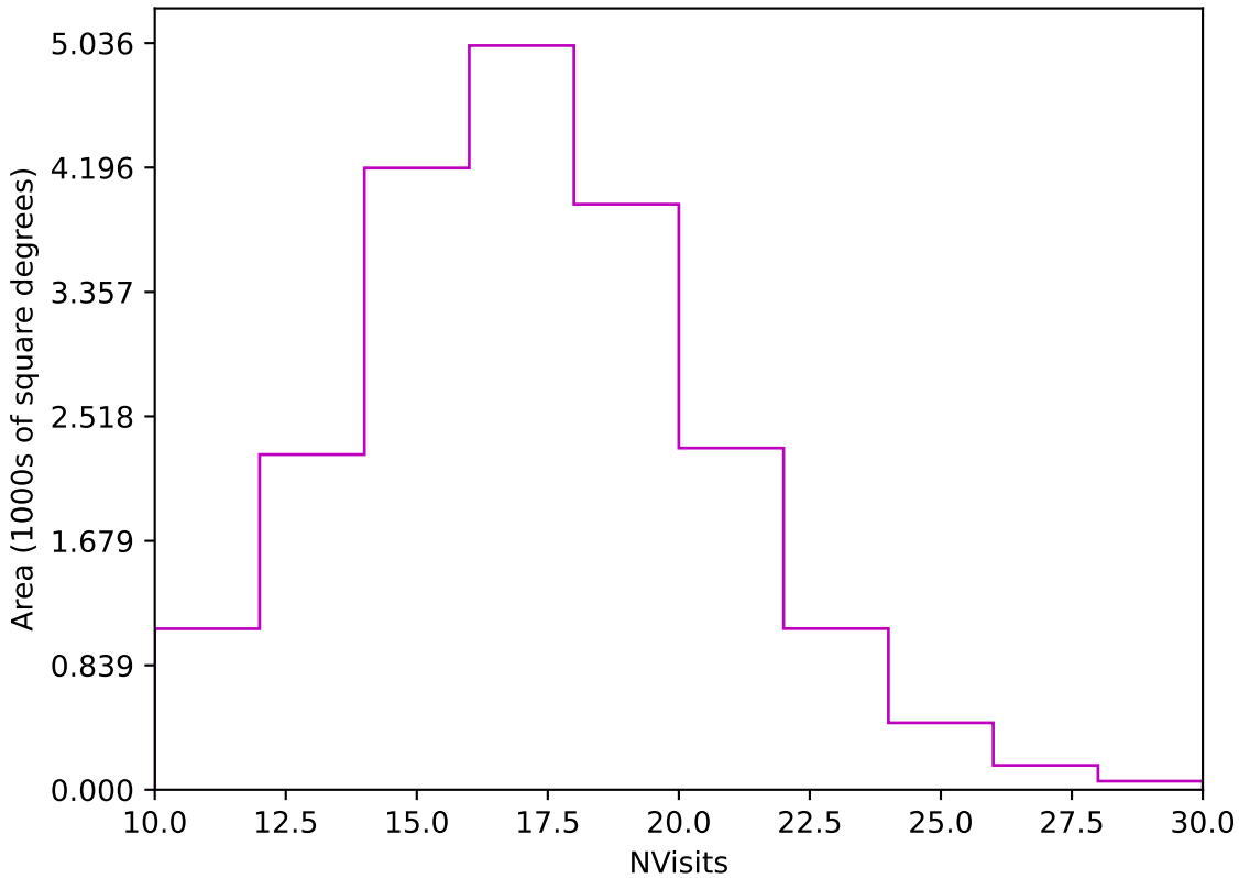
ddf_half_v3.4_10yrs Yr 1 z band: NVisits
