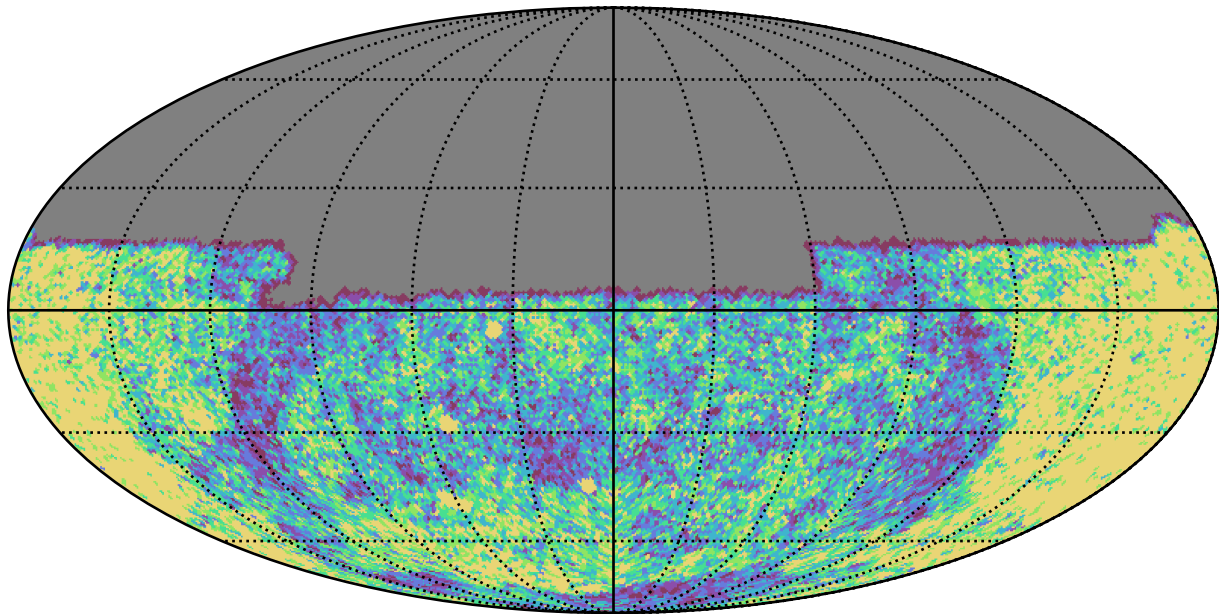
ddf_half_v3.4_10yrs Yr 1 u band: NVisits
