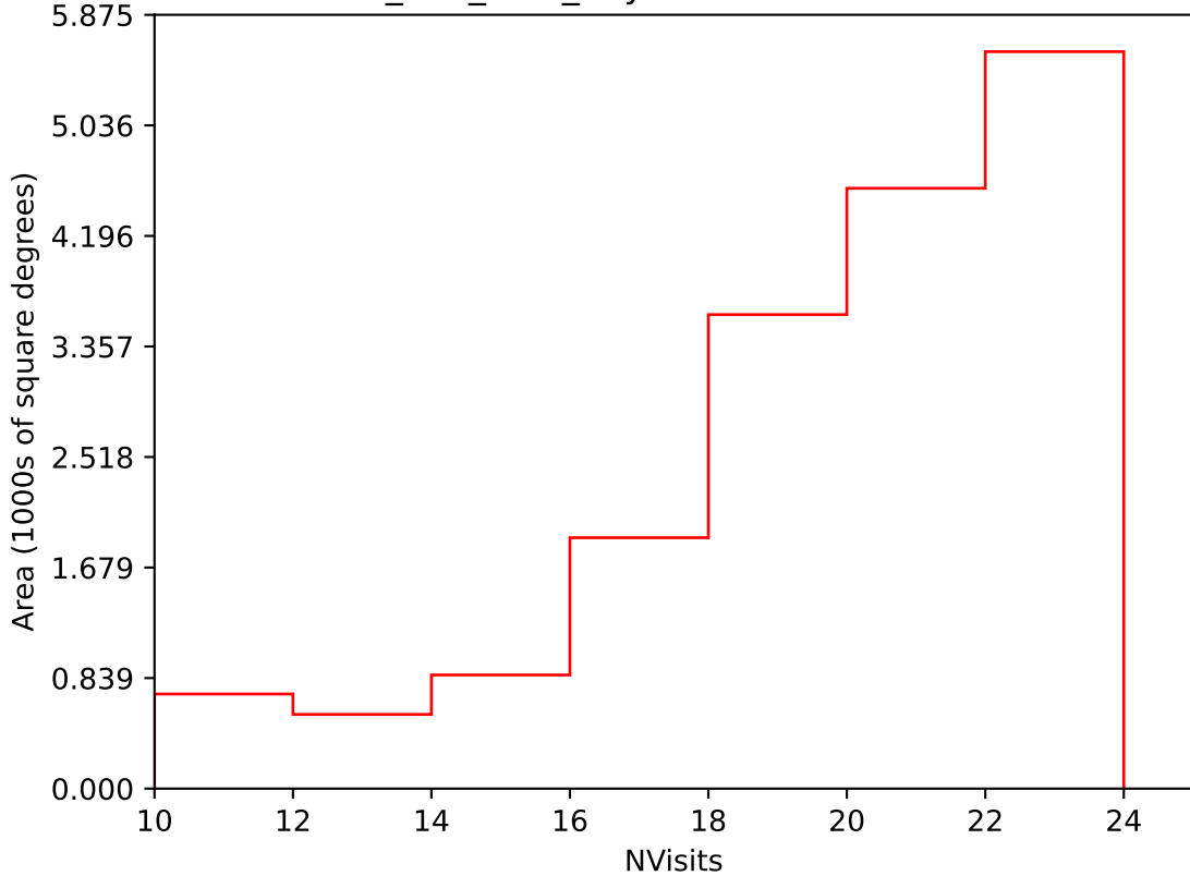
ddf_half_v3.4_10yrs Yr 1 i band: NVisits
