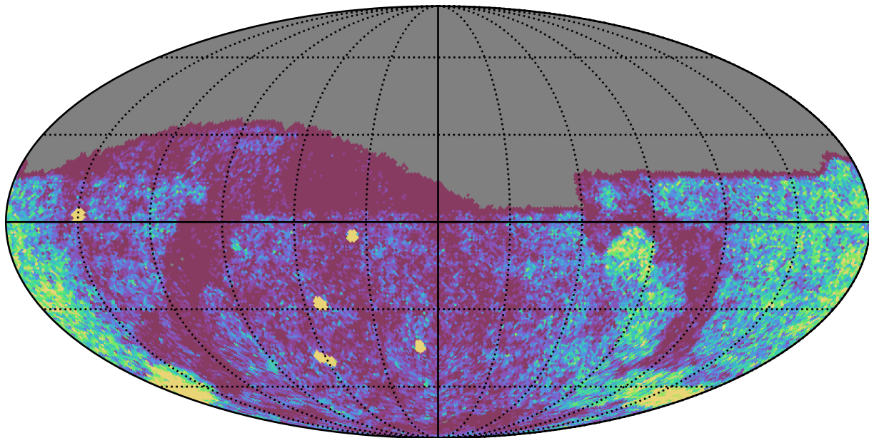
ddf_half_v3.4_10yrs Yr 1 g band: NVisits
