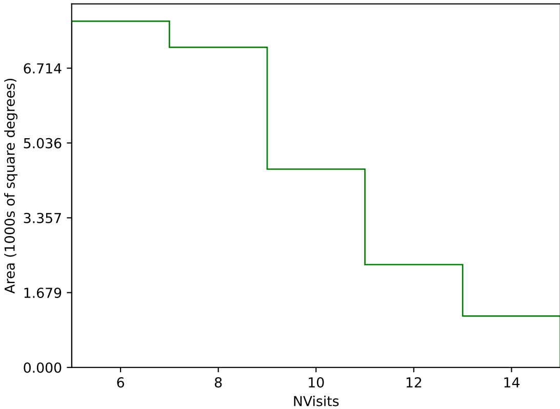
ddf_half_v3.4_10yrs Yr 1 g band: NVisits
