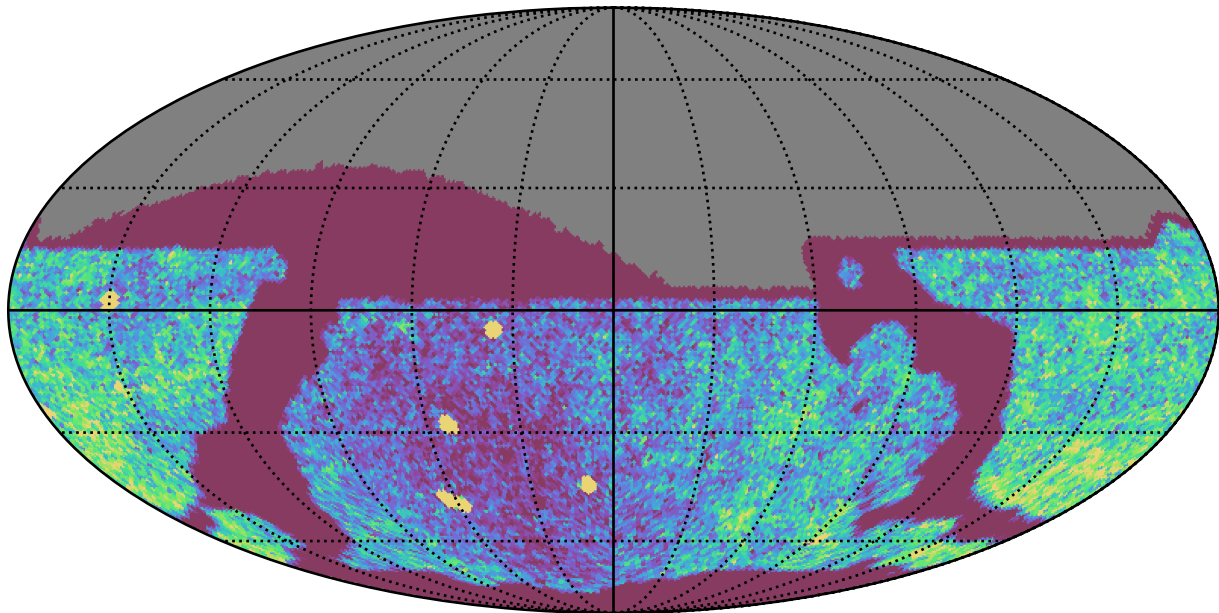
ddf_half_v3.4_10yrs Yr 1 all bands: NVisits
