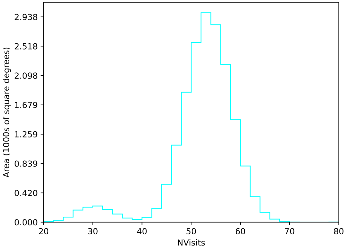
ddf_half_v3.4_10yrs WFD u band: NVisits
