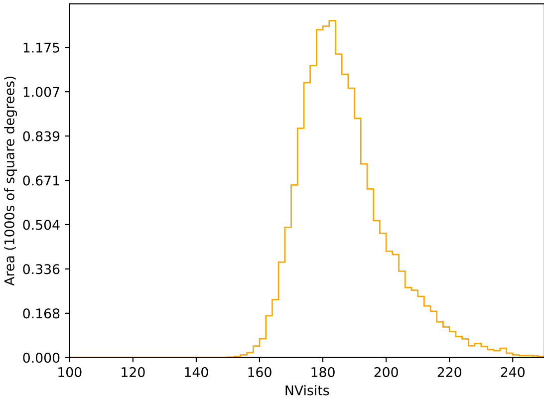
ddf_half_v3.4_10yrs WFD r band: NVisits
