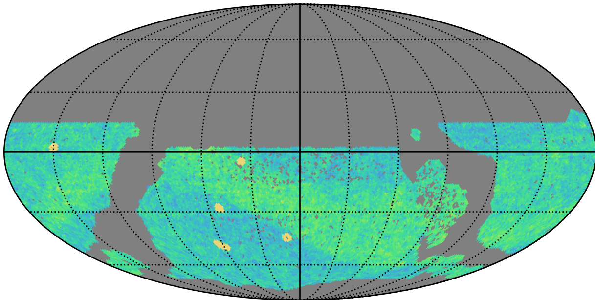
ddf_half_v3.4_10yrs WFD i band: NVisits
