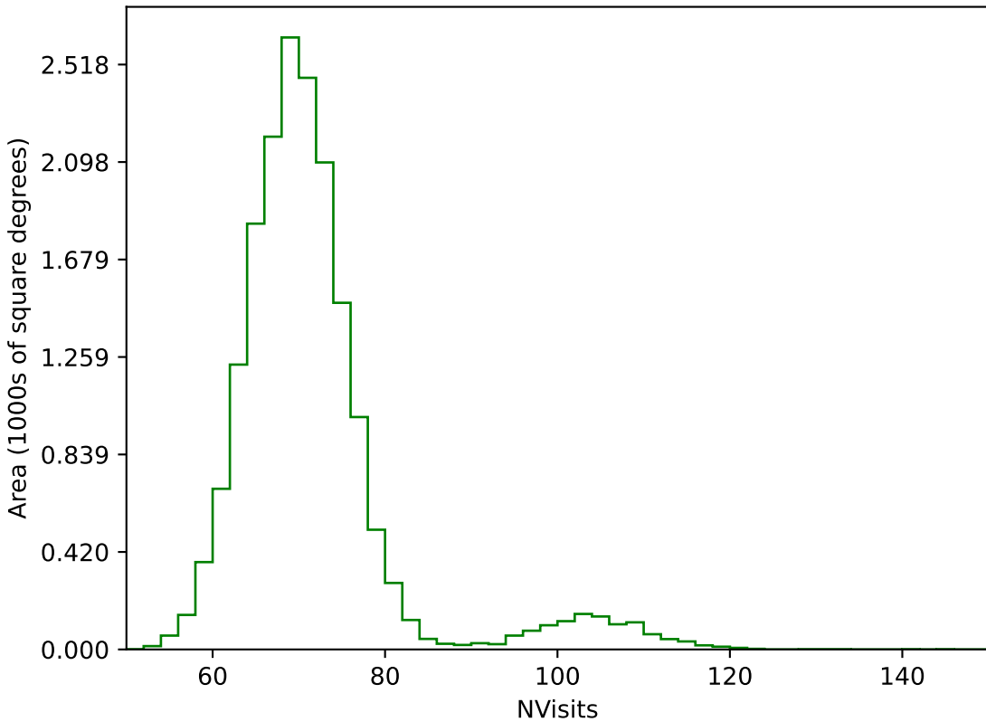
ddf_half_v3.4_10yrs WFD g band: NVisits
