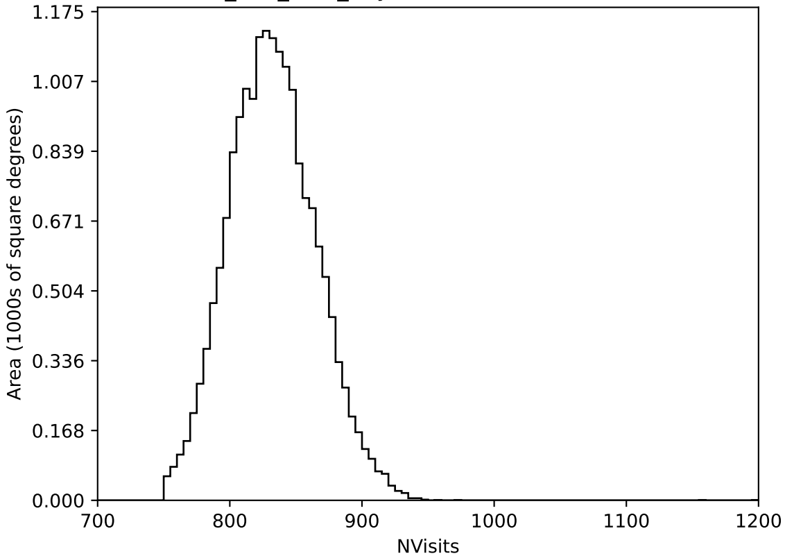
ddf_half_v3.4_10yrs WFD all bands: NVisits
