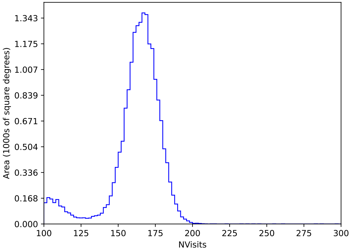
ddf_half_v3.4_10yrs All sky y band: NVisits
